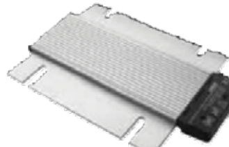
Electric Heater 230V, 380Watts Size 198×297mm
