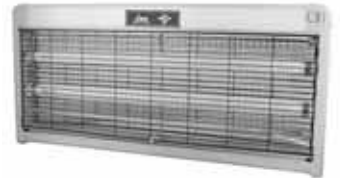
Fly Catcher Size: 610×60×270mm, 40W Size: 505×60×270mm, 30W Size: 395×60×270mm, 20W
